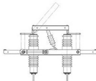
PVФз 10/630 III-III
