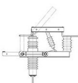
PVФз 10/630 II-II
