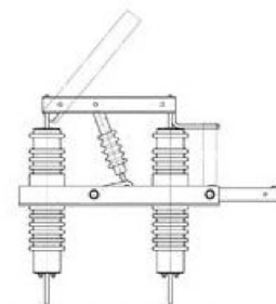
PVФз 10/630 I-III
