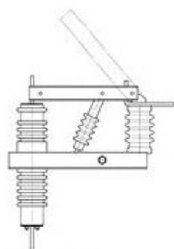
PVФз 10/630 I
