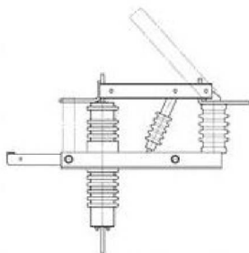
PVФз 10/630 I-I
